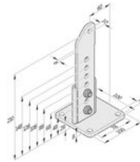
Post bracket 60/120 S10751-00001
