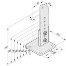
Post bracket 60/120 S10755-00001
